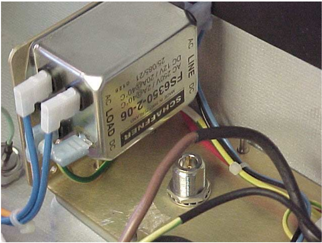
AC_DC Filter
