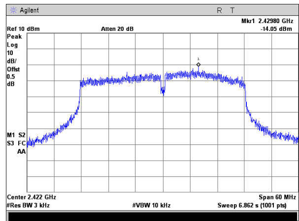
(802.11n40) channel 3
