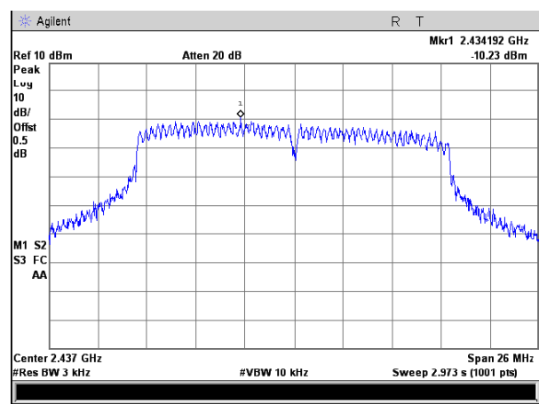
(802.11g) channel 6
