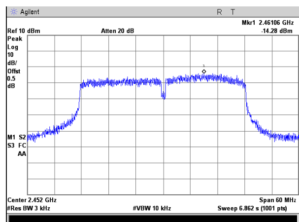
(802.11n40) channel 9
