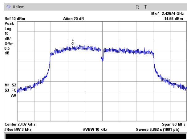
(802.11n40) channel 6
