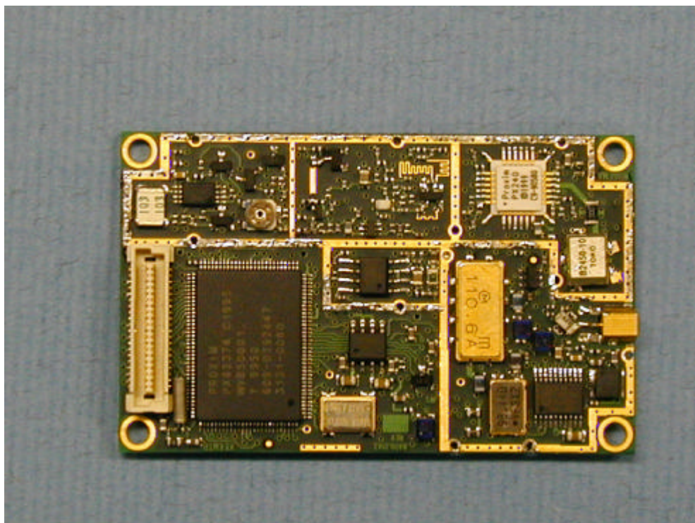
Circuit Board without shield (Front)
