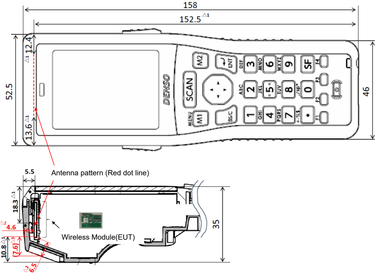
Antenna location
