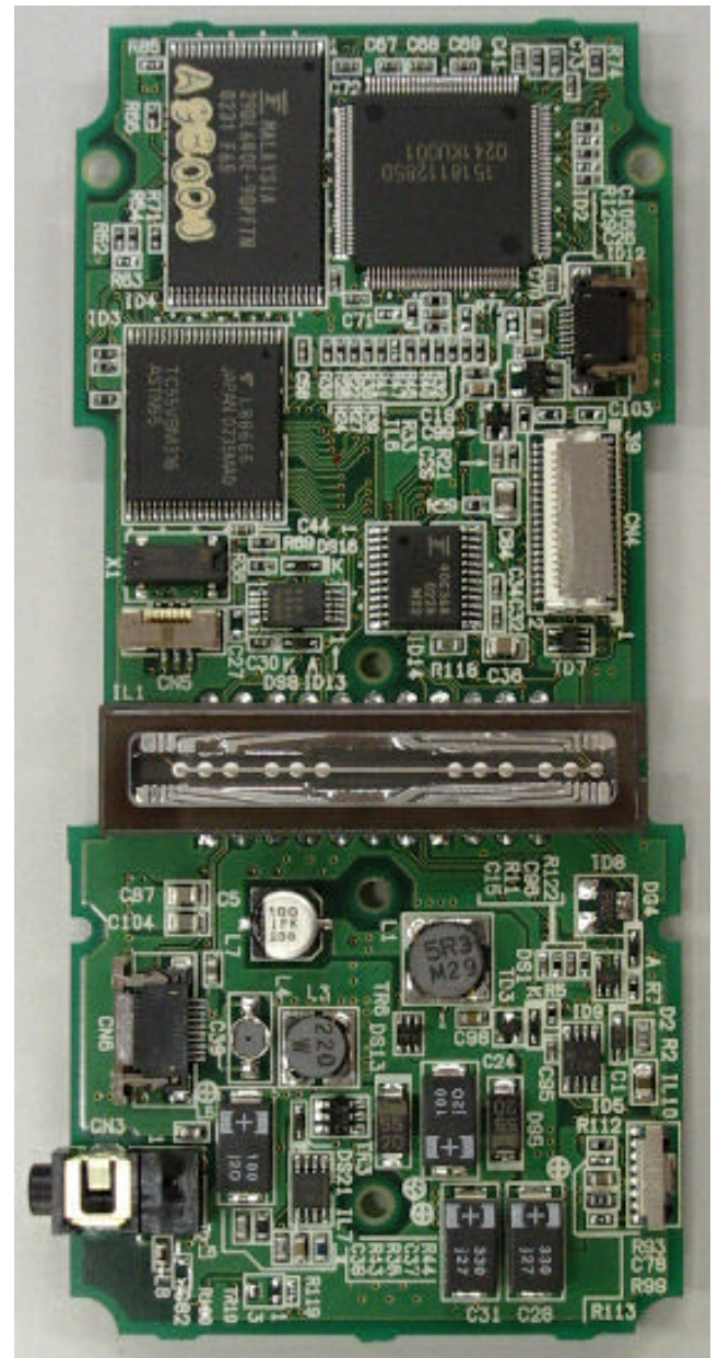
Solder Side
