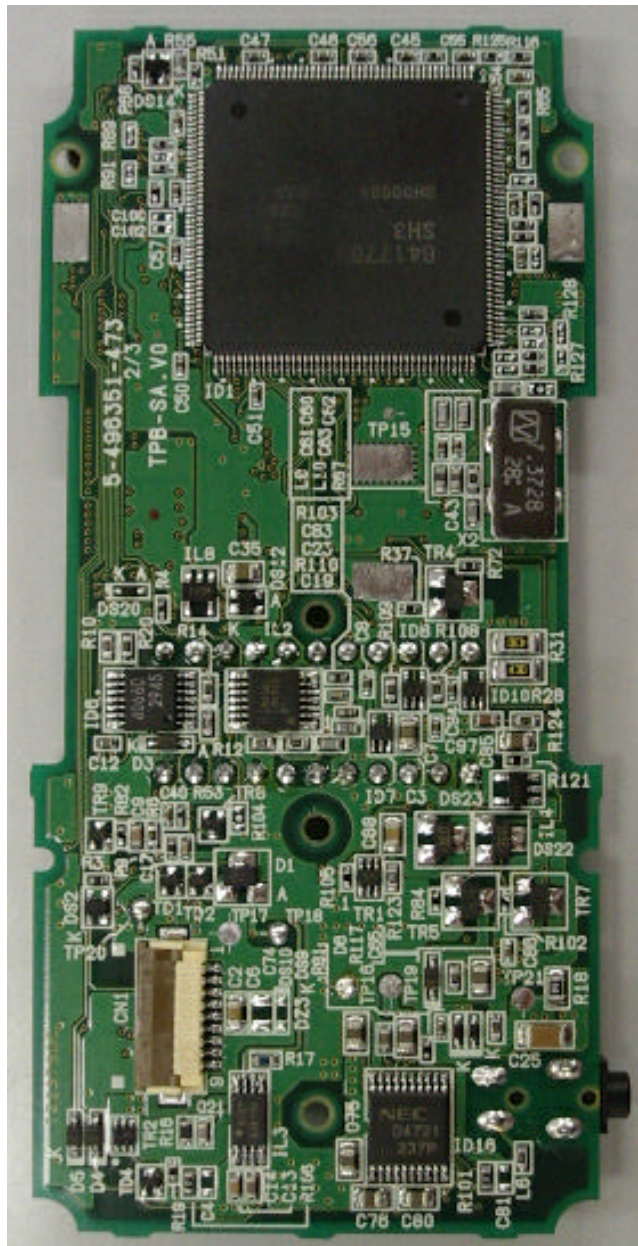
Component Side
