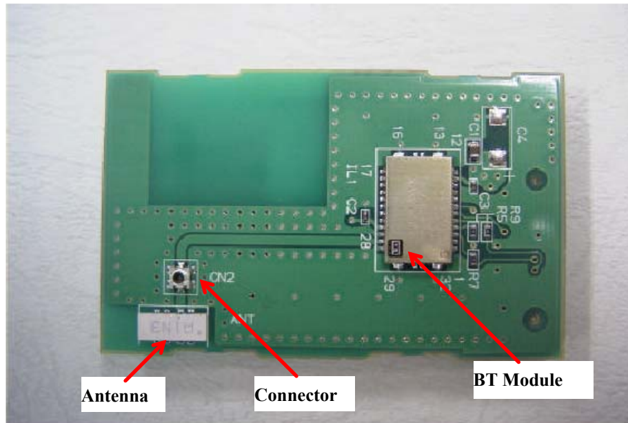
Photo of Bluetooth Board (Solder side)
