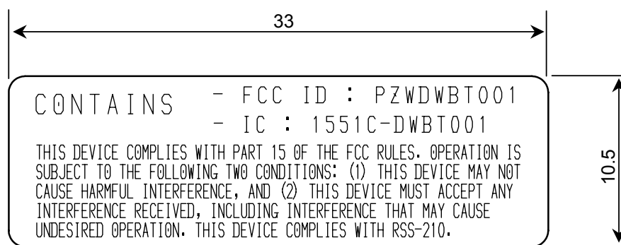
Fig. 4.6.2. FCC and IC ID Label layout
