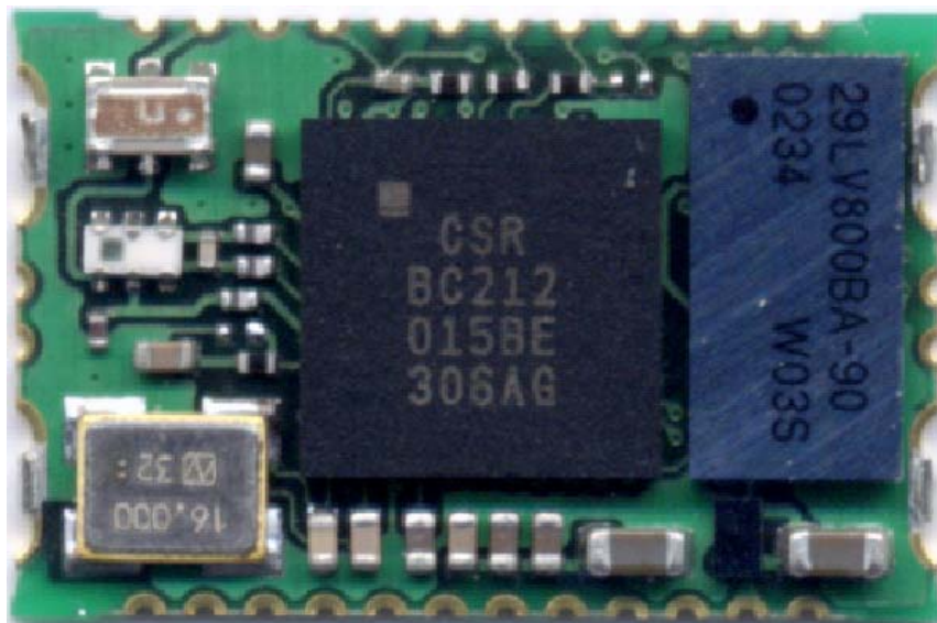
Internal Photo of Bluetooth Module IC (Component side)
