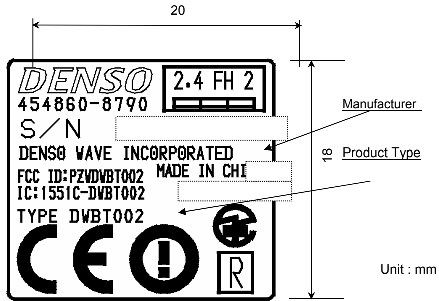
Fig. Label Layout
