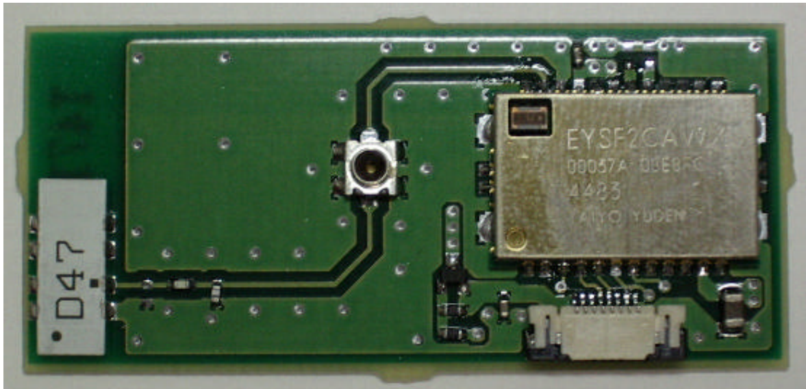
Photo. Bluetooth Board (Component Side)
