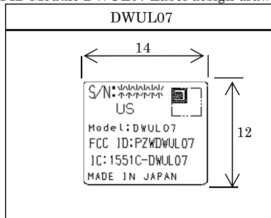
RFID Module DWUL07 Label design drawing
