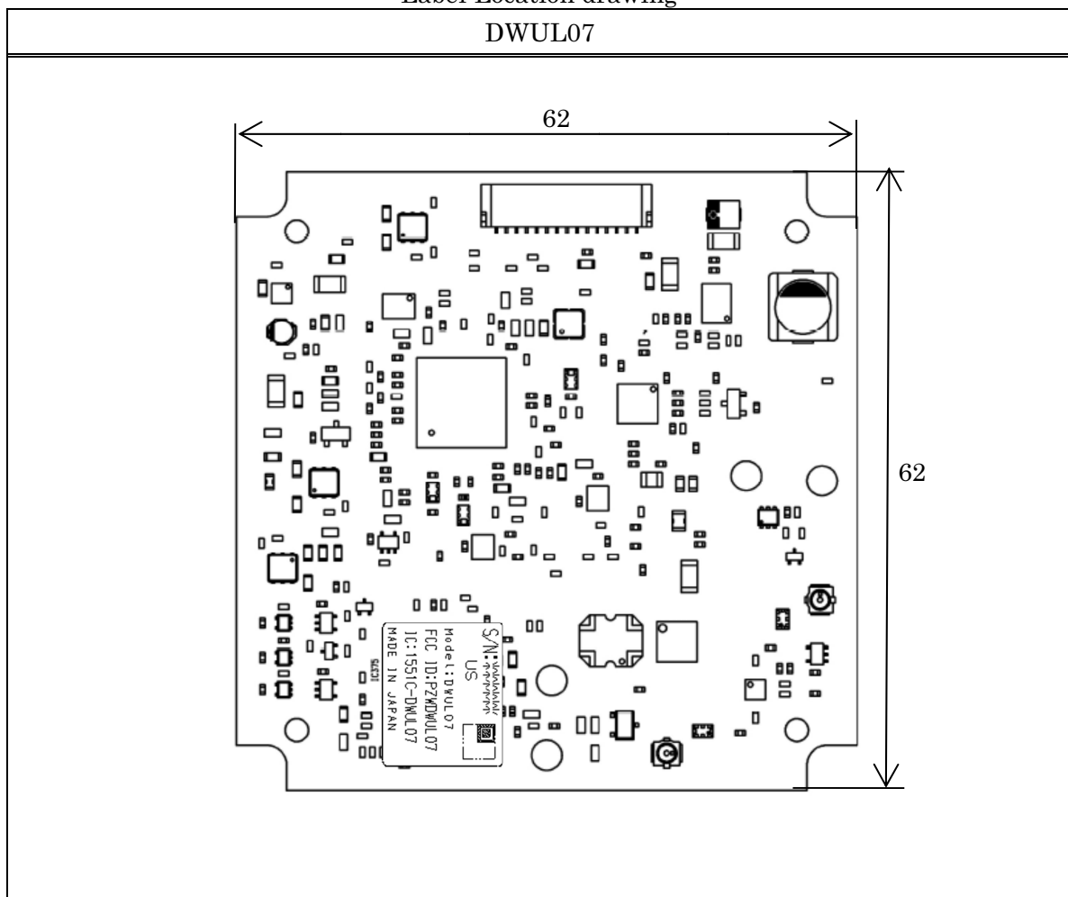
Label Location drawing
