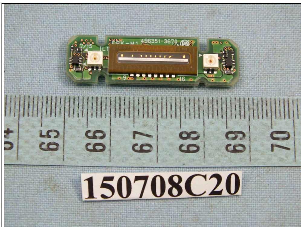
Specific End-product (Handy Terminal): BHT-1461QWB-CE
