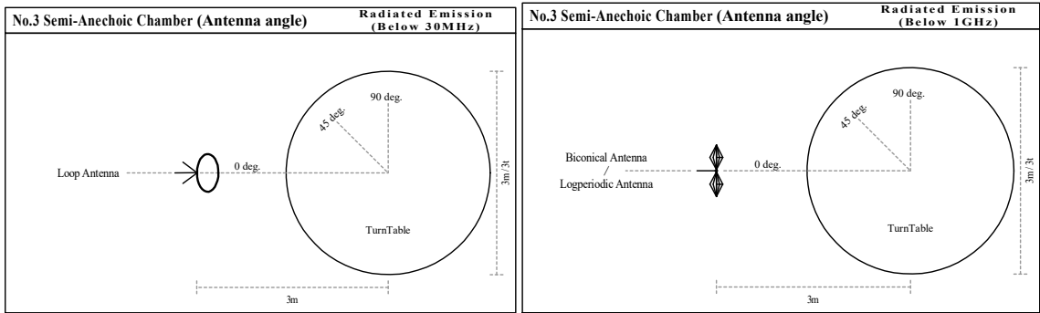
Figure 2. Antenna angle
