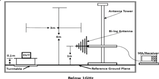
Figure 2. 30MHz to 1GHz
