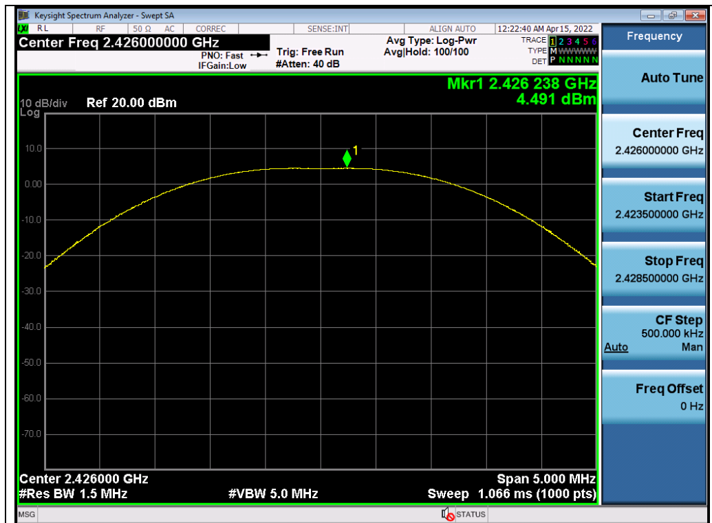
Test_Graph_LE1M_ANT1_2426_1Mbps_Peak Power
