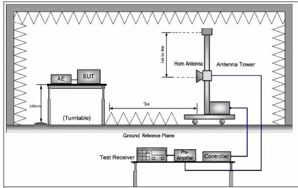
Figure 3. Above 1 GHz
