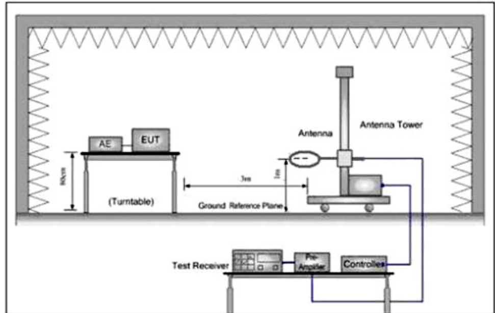
Figure 1. Below 30MHz
