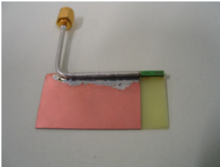
Picture 2 : External antenna (size of the ground plane of 40 x 25 mm)
