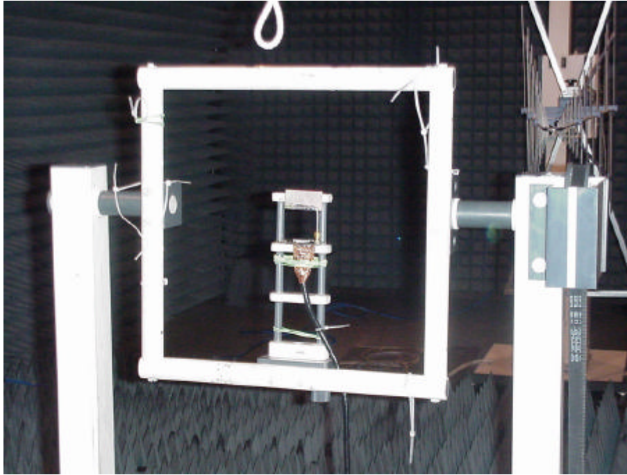
Picture 3 : setup for the test "Spurious emissions radiated"
