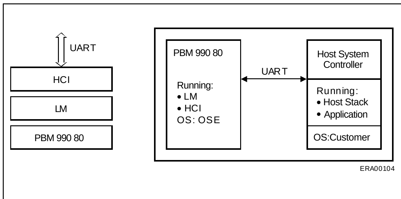
Figure 6 Host Controller Interface
