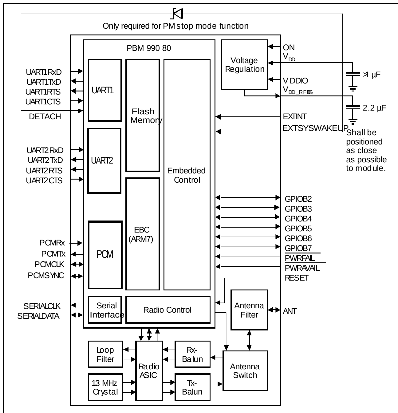
Figure 2 Block Diagram
