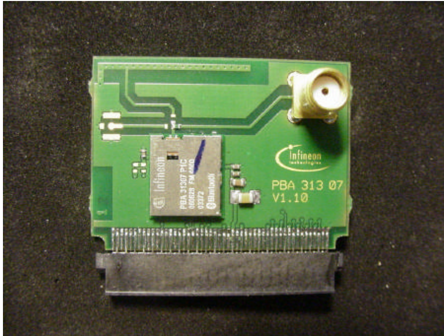
Picture 1 : EUT (front view)
