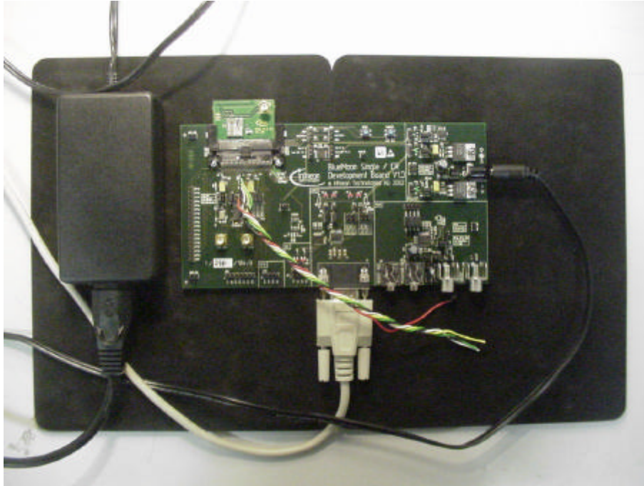
Picture 3 : setup for conducted tests
