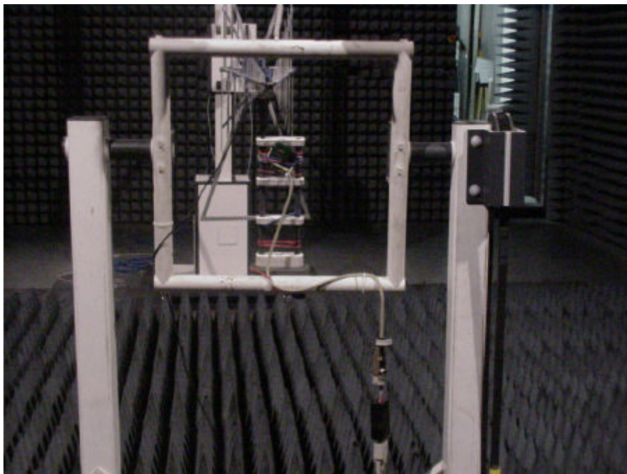
Picture 4 : setup for spurious emissions radiated tests
