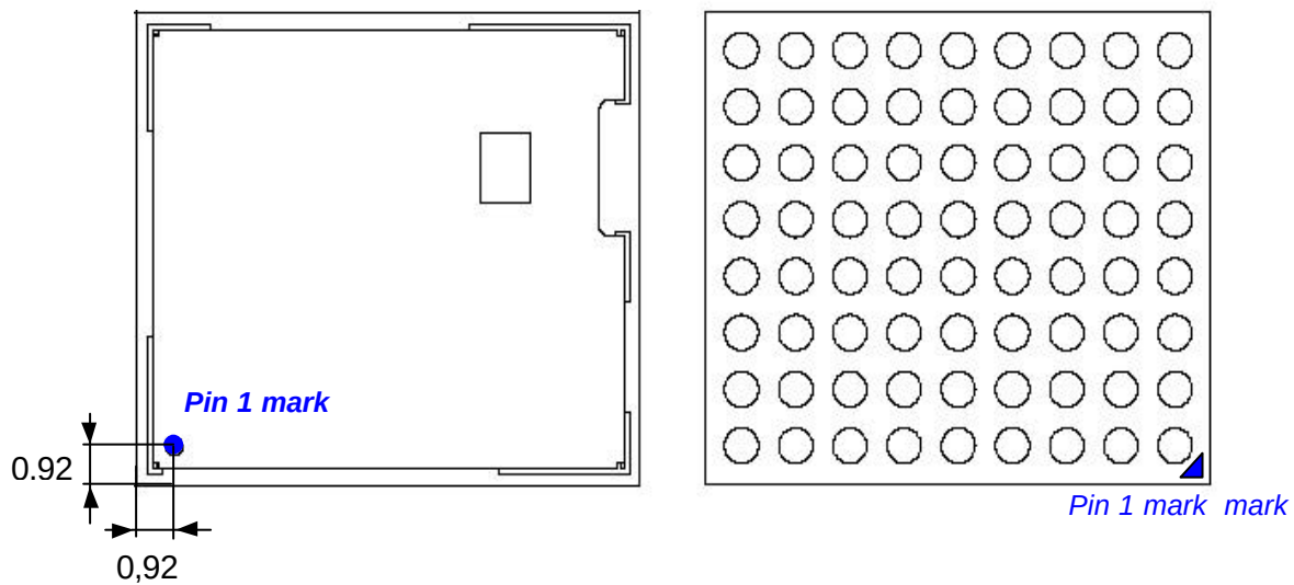
Figure 4-2 Pin mark
