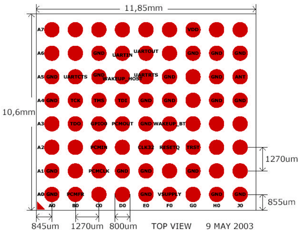
Figure 4-1 Pad layout on the module (top view)
