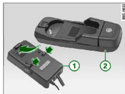
Fig. 98 Installing the adapter
