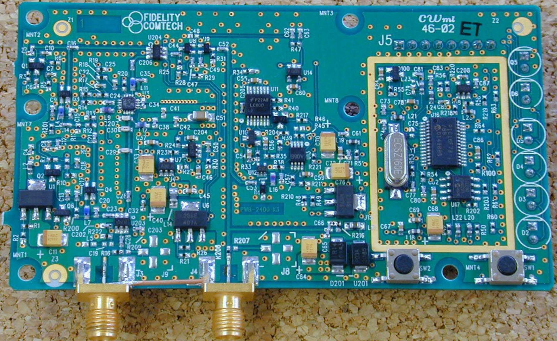
FCI-2451 Amplified Antenna (Witch's Hat) - PCB (Top) (Identical to FCI-2401)
