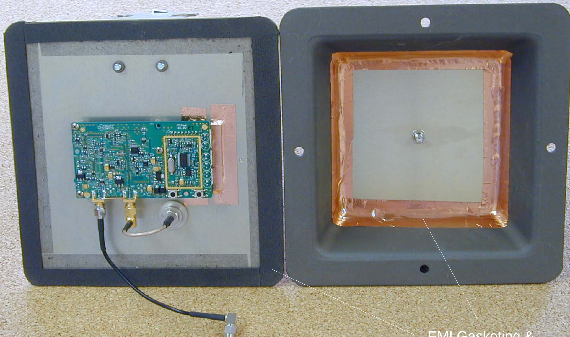
FCI-2451 Amplified Antenna (Witch's Hat) - Case Open (1)
