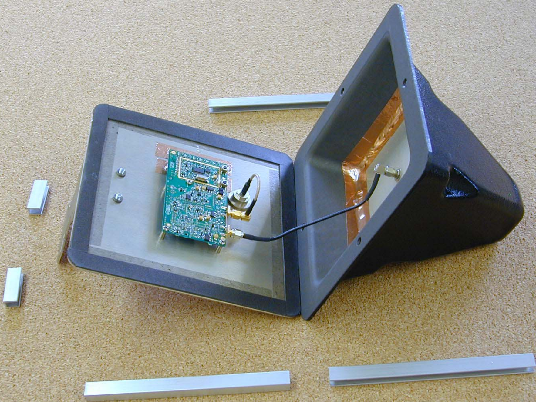
FCI-2451 Amplified Antenna (Witch's Hat) - Case Open (2)
