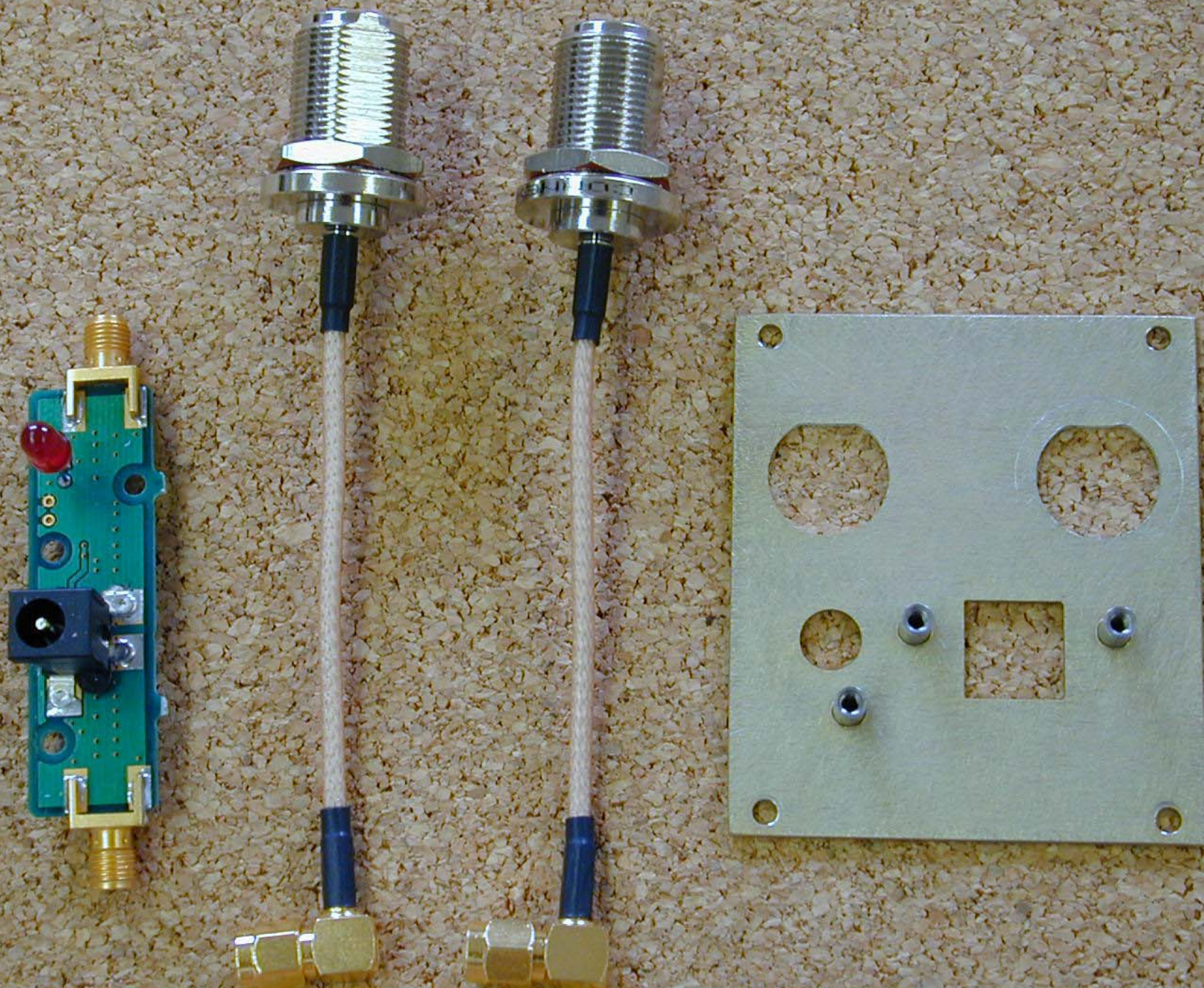
DC Power Injector - Mount Apart (top)
