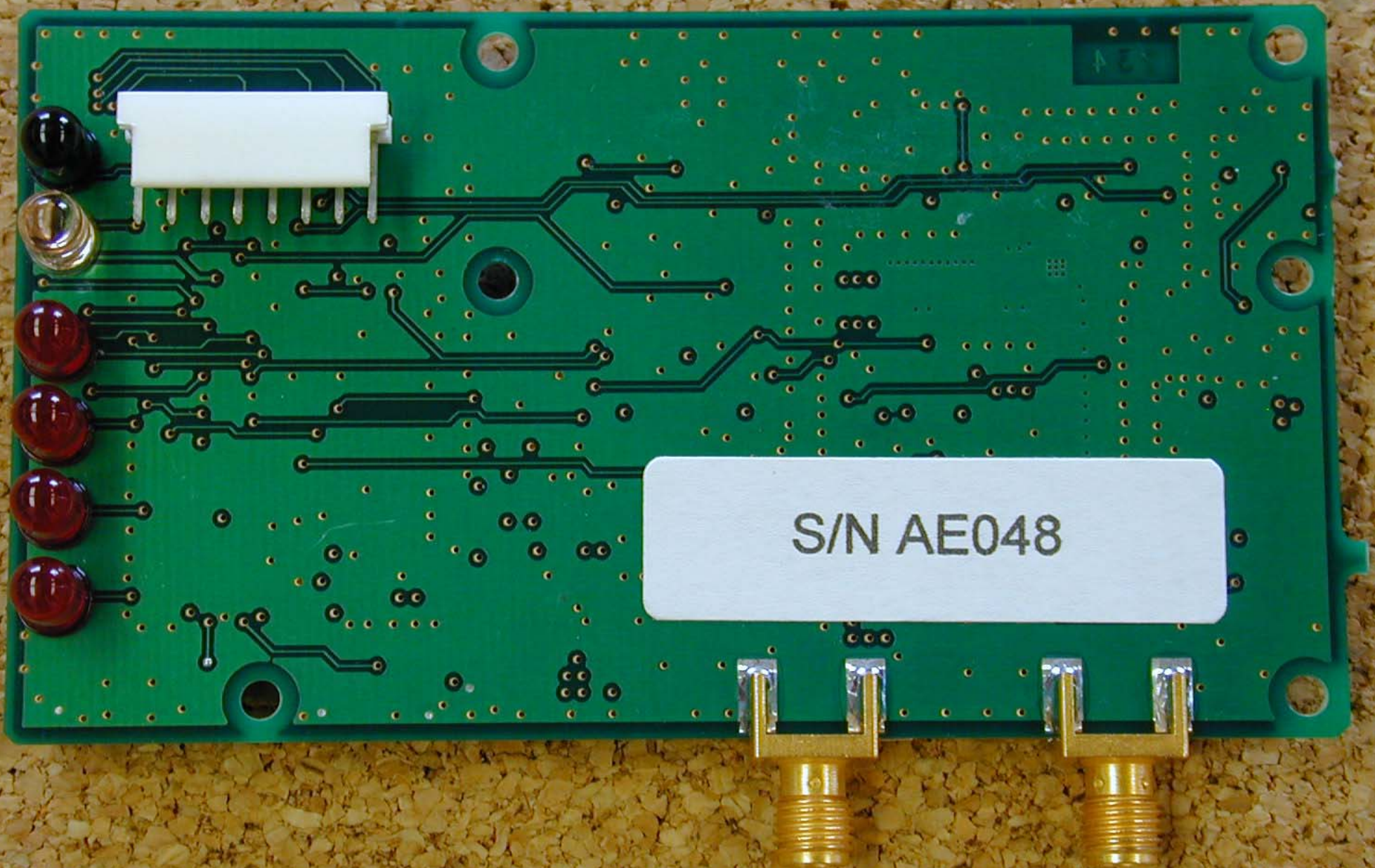
FCI-2451 Amplified Antenna (Witch's Hat) - PCB (Bottom) (Identical to FCI-2401)
