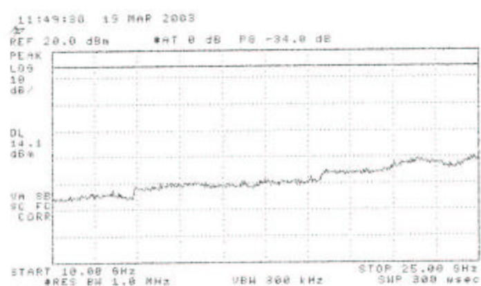
Figure 6.11 Antenna conducted spurious emissions. (low, mid, & high channels – 100 mW, 10dB Pad)
