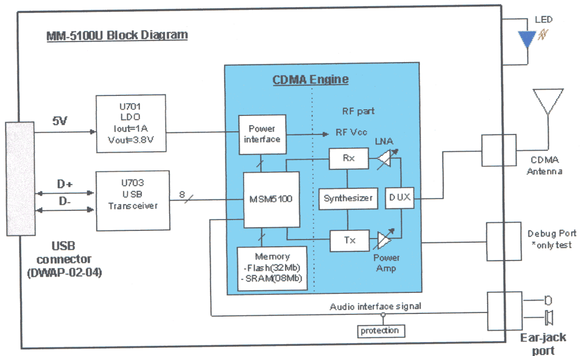
Figure 4.1 MM-5100U CDMA 1X modem block diagram
