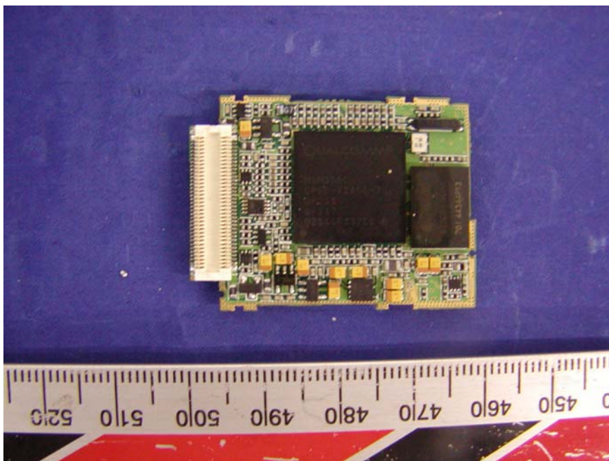
Main Board – Bottom Cover Removed View
