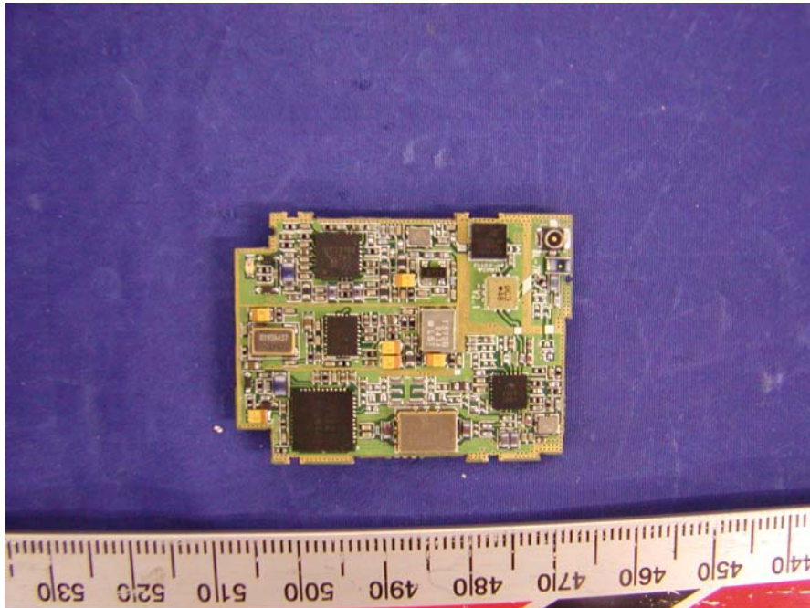
Main Board – Top Cover Removed View
