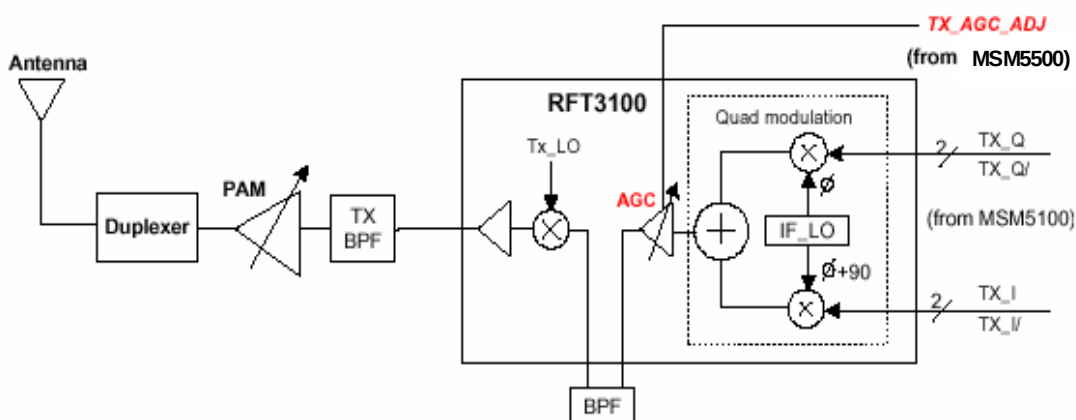
Figure 9. Output Circuit
