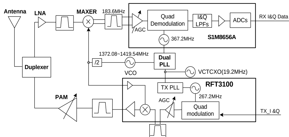
Figure 10. Frequency determining and stabilizing and circuitry 20/20
