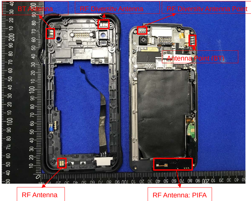
EUT UNCOVER VIEW 2
