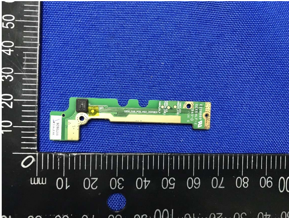
CIRCUIT REAR1 REAR VIEW
