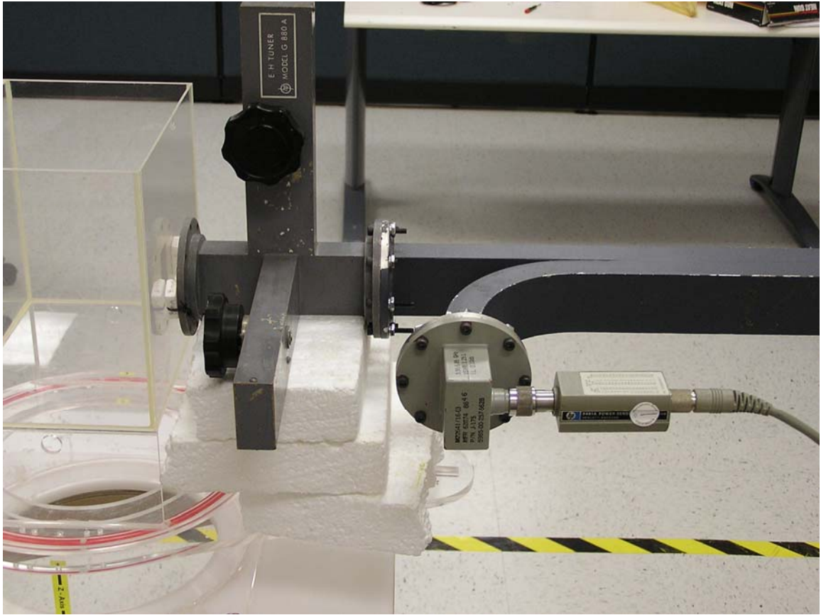
WG_setup2
