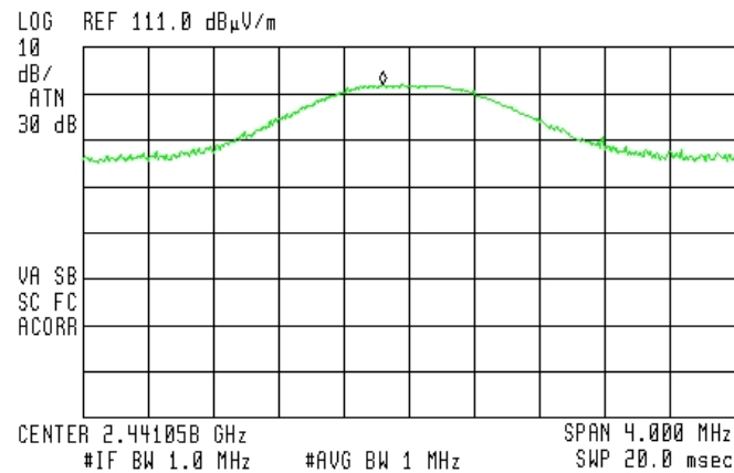
Figure 19 2441 MHz
