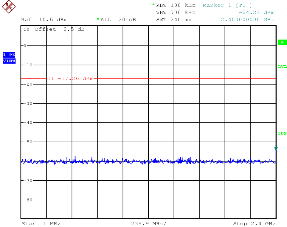
Bluetooth 4.0, Lowest Channel, Plot A
