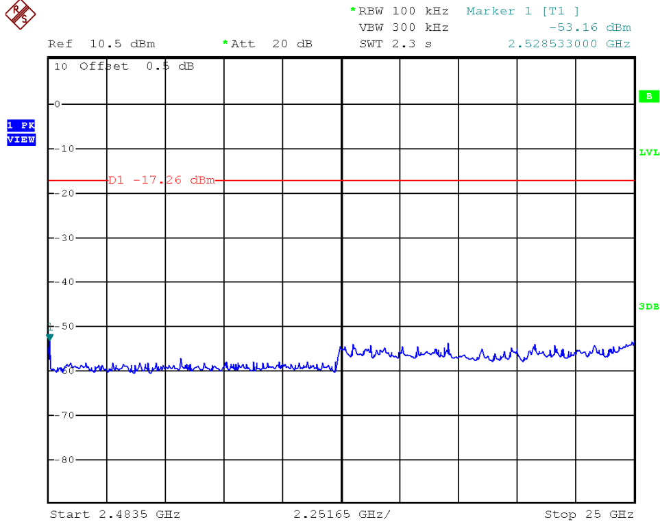
Bluetooth 4.0, Lowest Channel, Plot B
