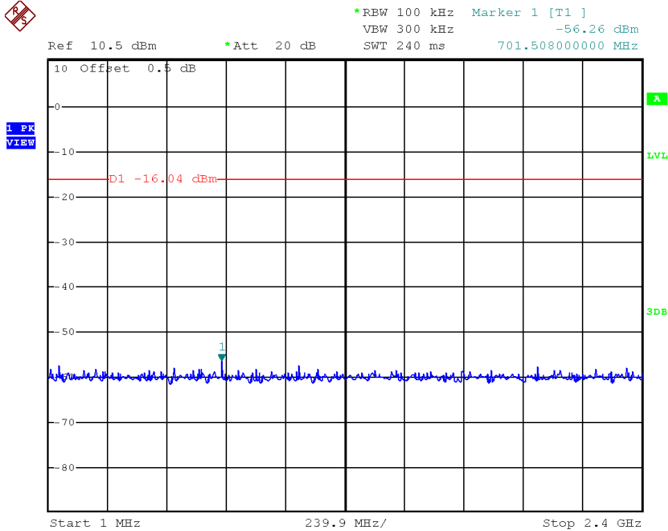
Bluetooth 4.0, Middle Channel, Plot A
