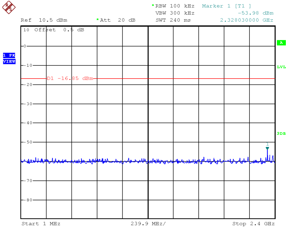
Bluetooth 4.0, Highest Channel, Plot A
