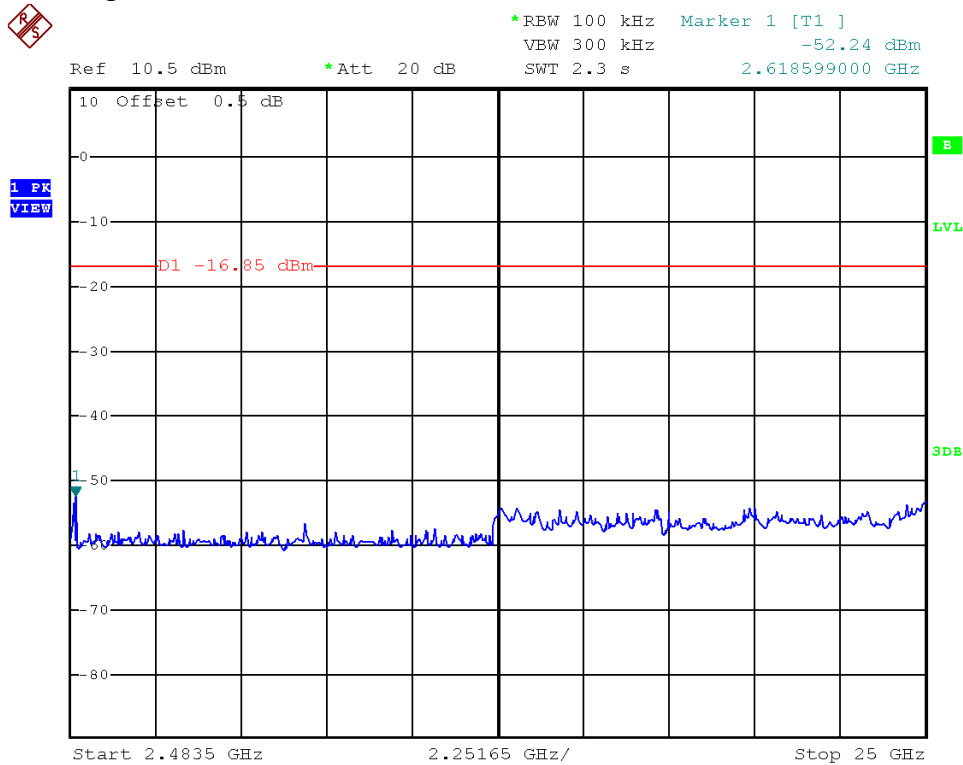
Bluetooth 4.0, Highest Channel, Plot B
