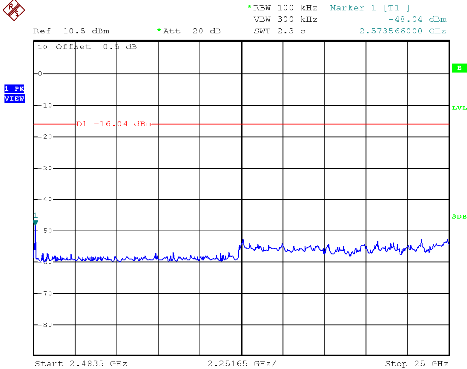
Bluetooth 4.0, Middle Channel, Plot B
