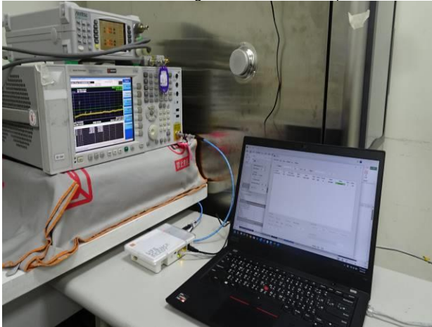
FCC_15_247_Zigbee_Radiated_Setup
