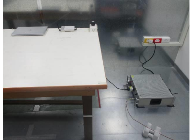
FCC_15_247_Zigbee_Conduction_Setup
