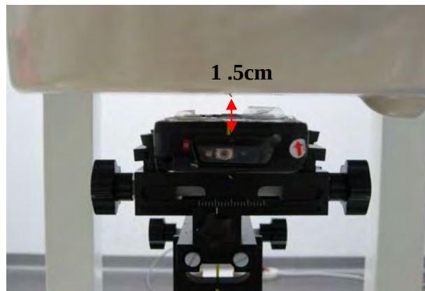
Fig.7 EUT front to flat phantom
