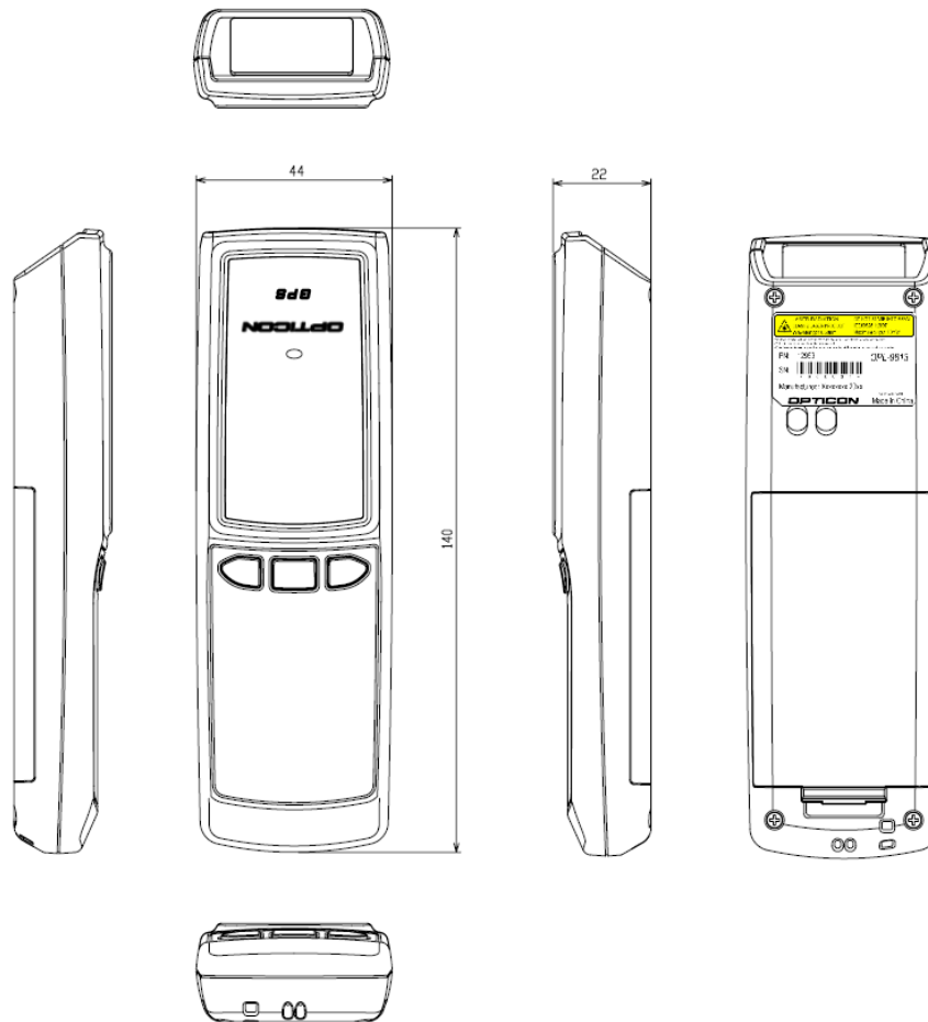
Figure 12: Mechanical drawing
