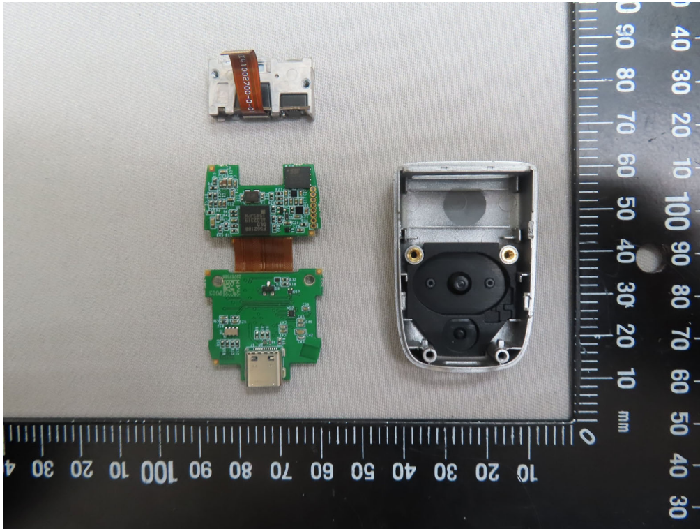
Inside View of EUT – 2
