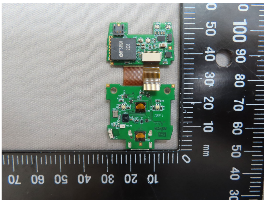
Inside View of EUT – 5
