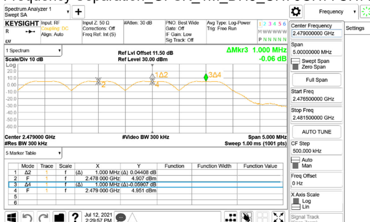
Frequency Separation_GFSK_1M_DH5_CH76CH77CH78
