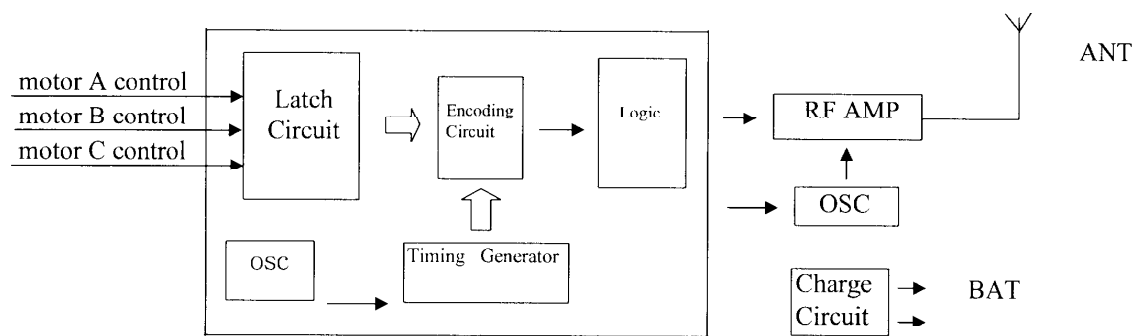
TX Block Diagram
