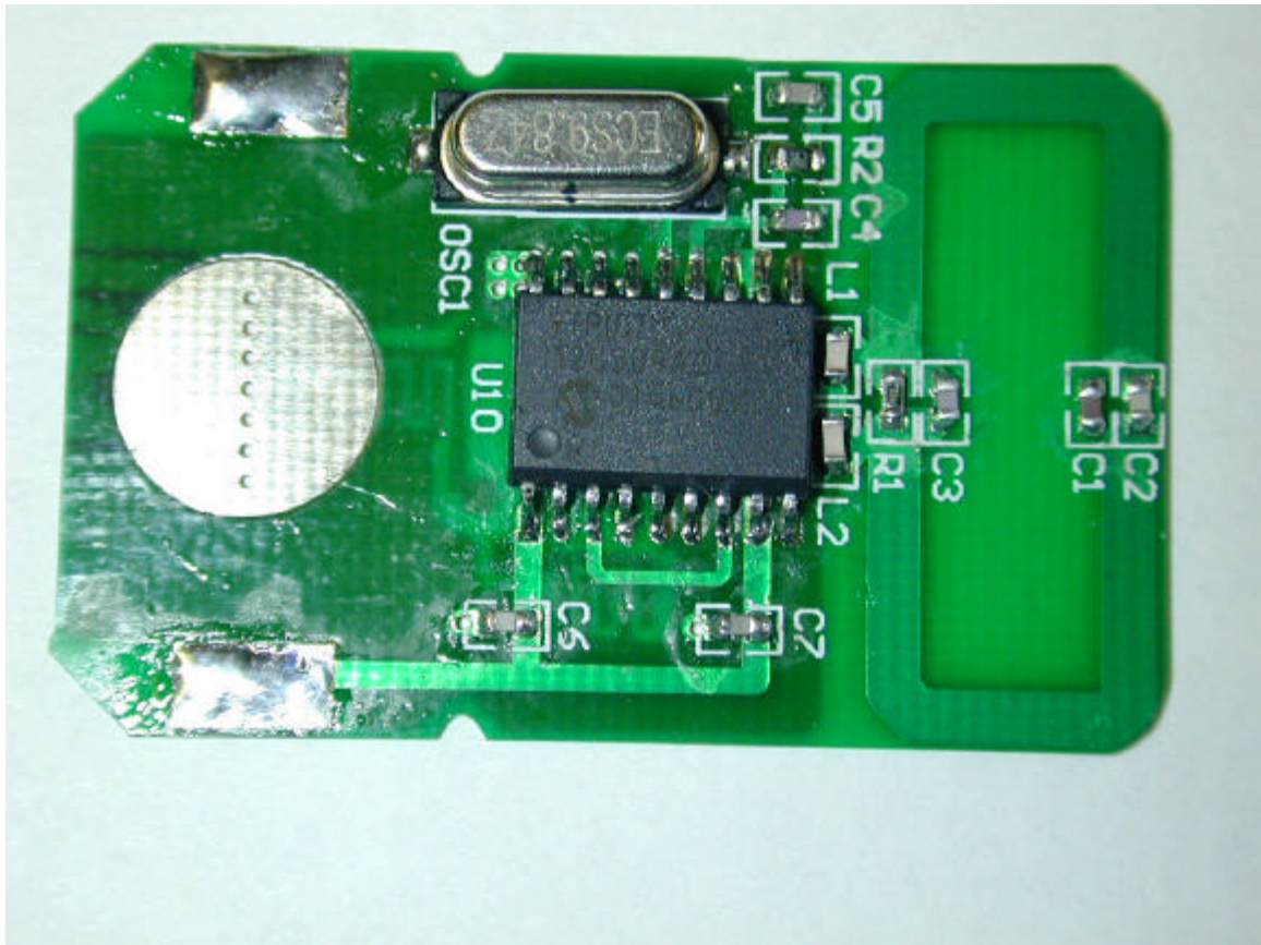
Internal Component Side View without Battery Holder
