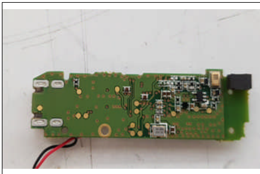
Bottom view of PCB
