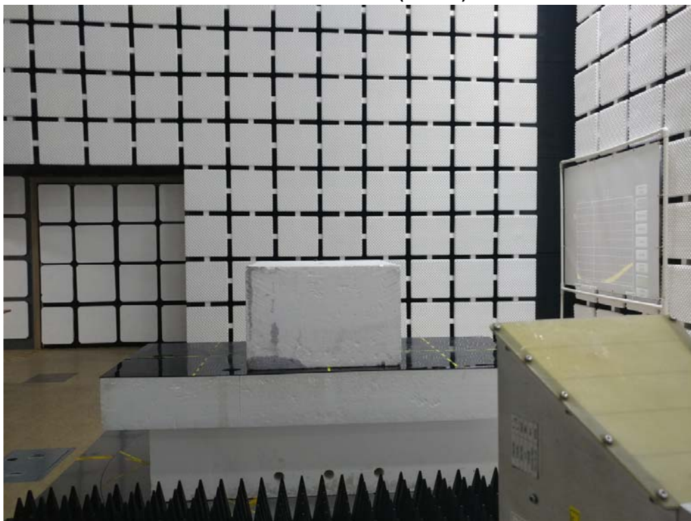
Radiated RF measurement (>1GHz) Left ear
