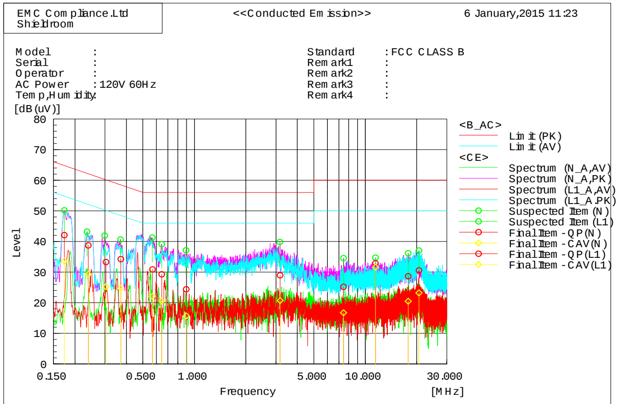
Figure 7. plot of Conducted Emission
