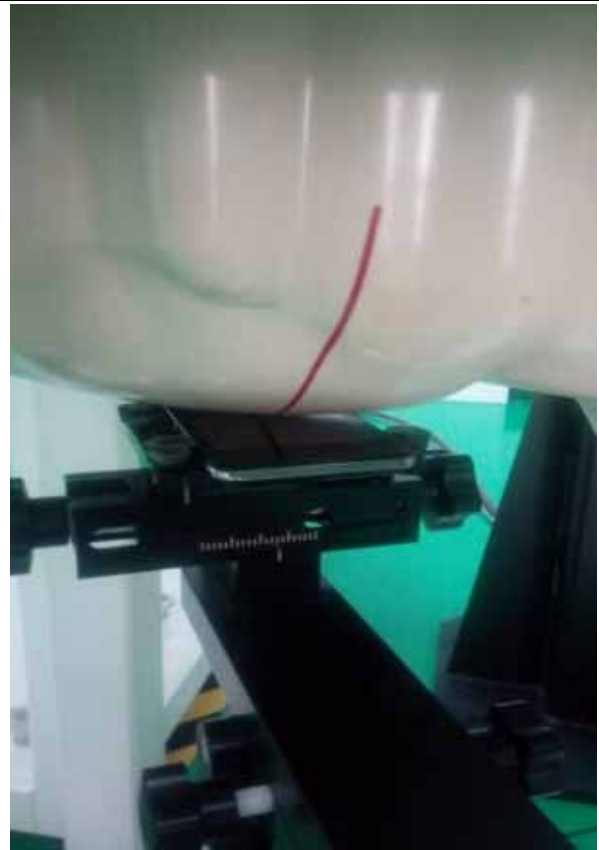
Right Cheek position
