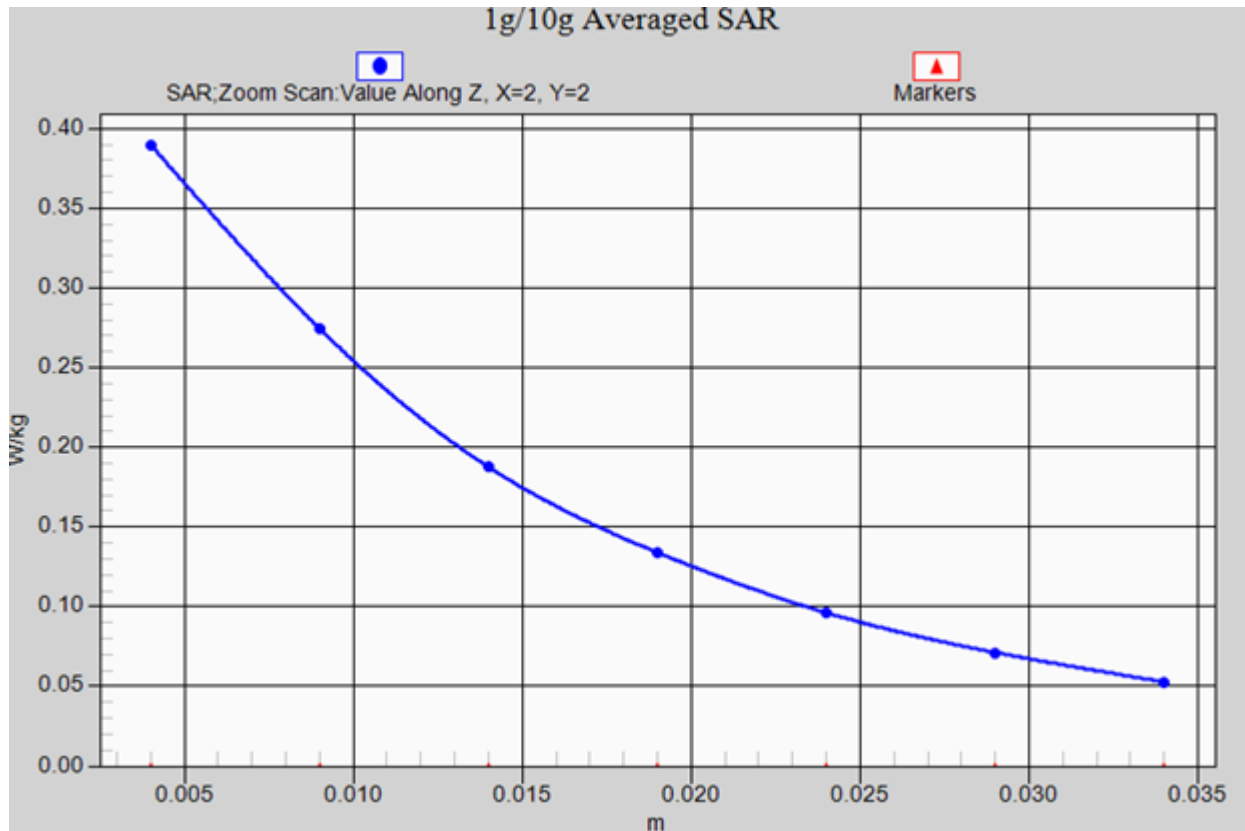
GSM850 LEFT/CHEEK-High- axis scan
