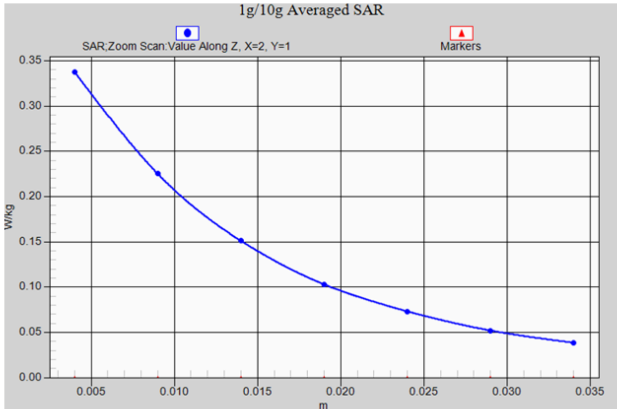
WCDMA Band V- LEFT/CHEEK-Low -axis scan
