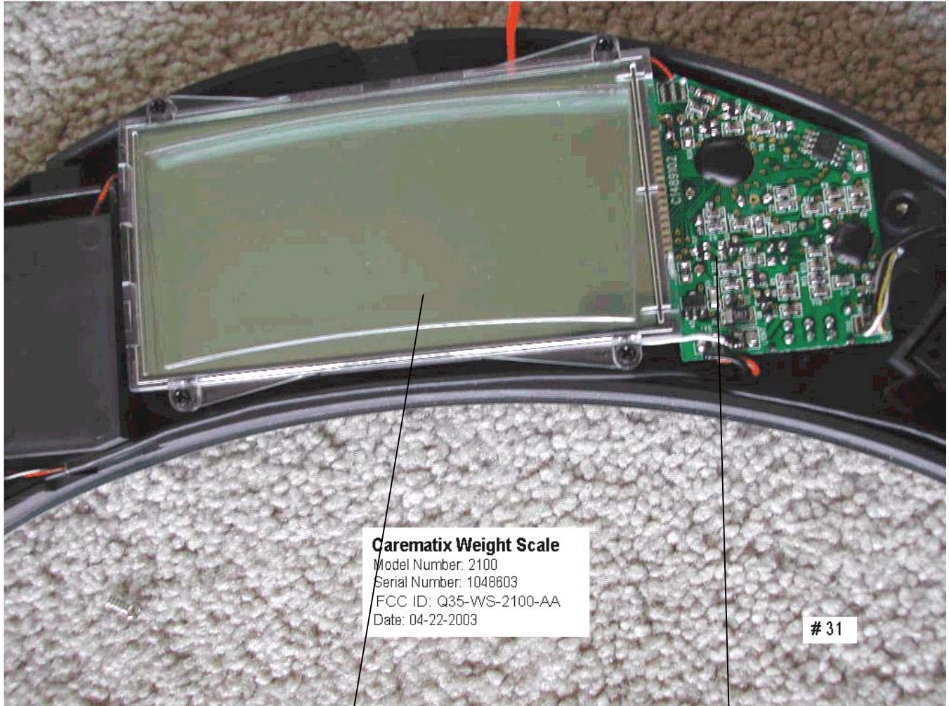
Weight Scale Primary Board (Top View)
