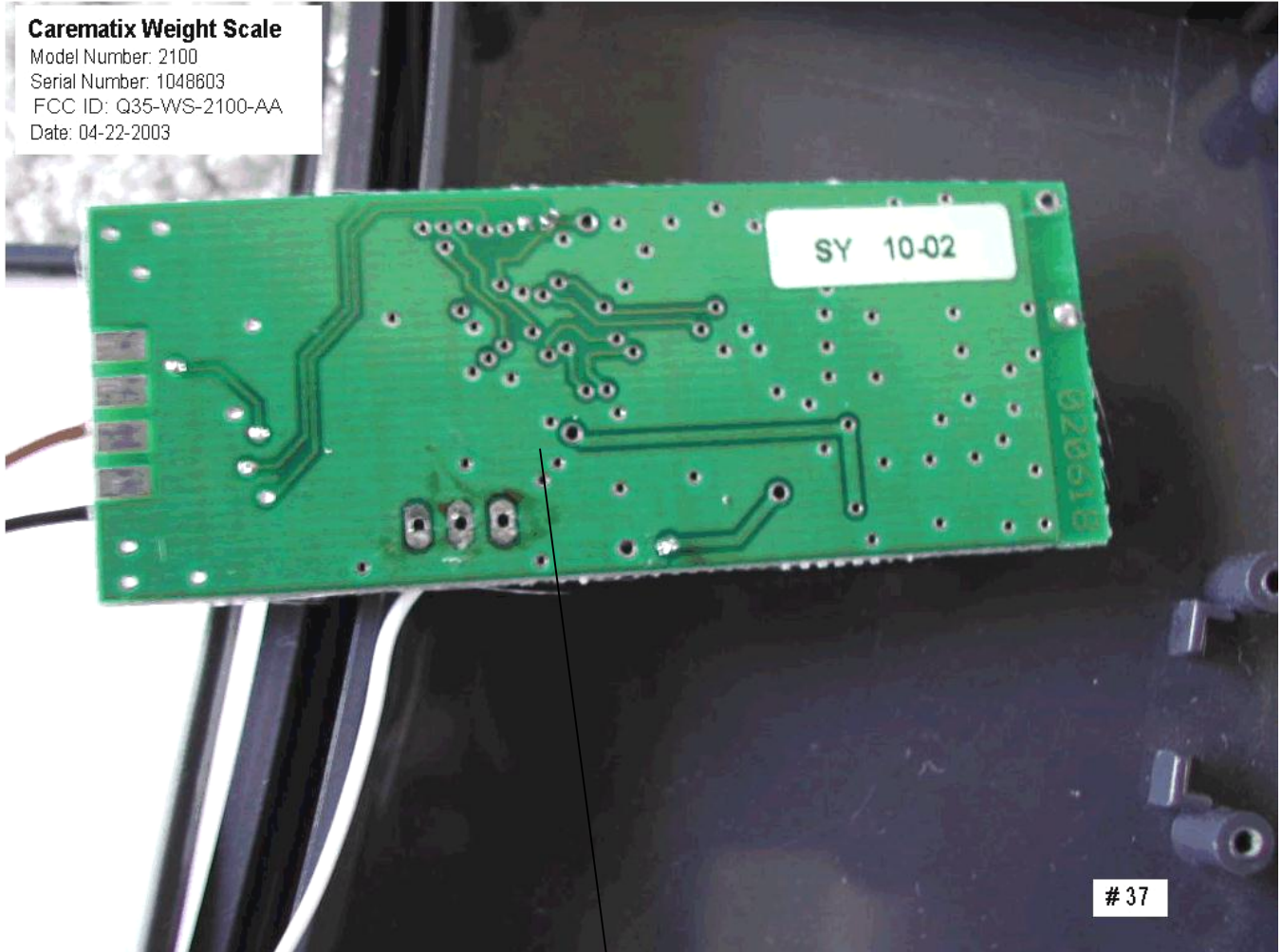
Transceiver (HUB4) Board (Bottom View)
