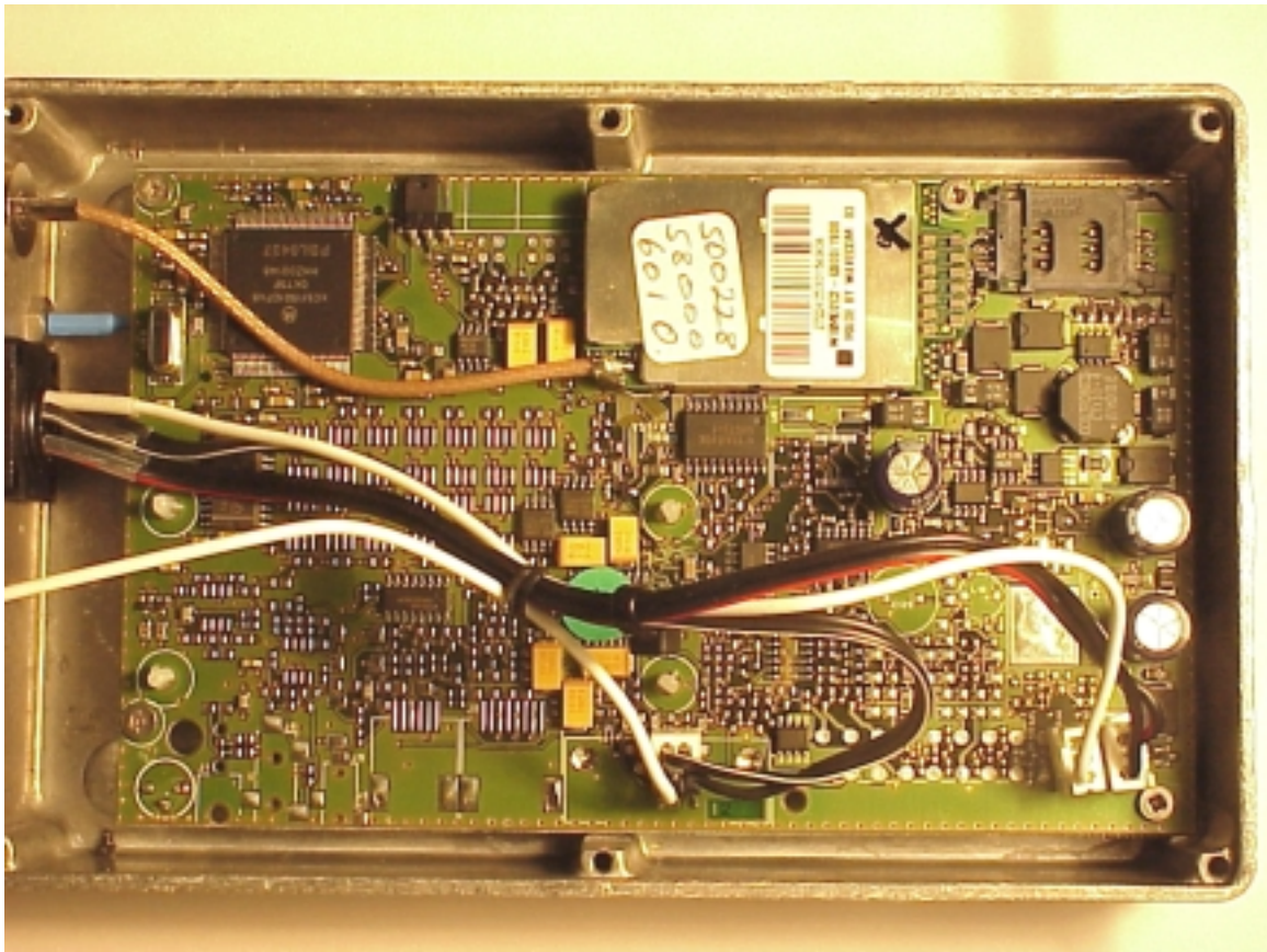
PCB – Top view shielded
