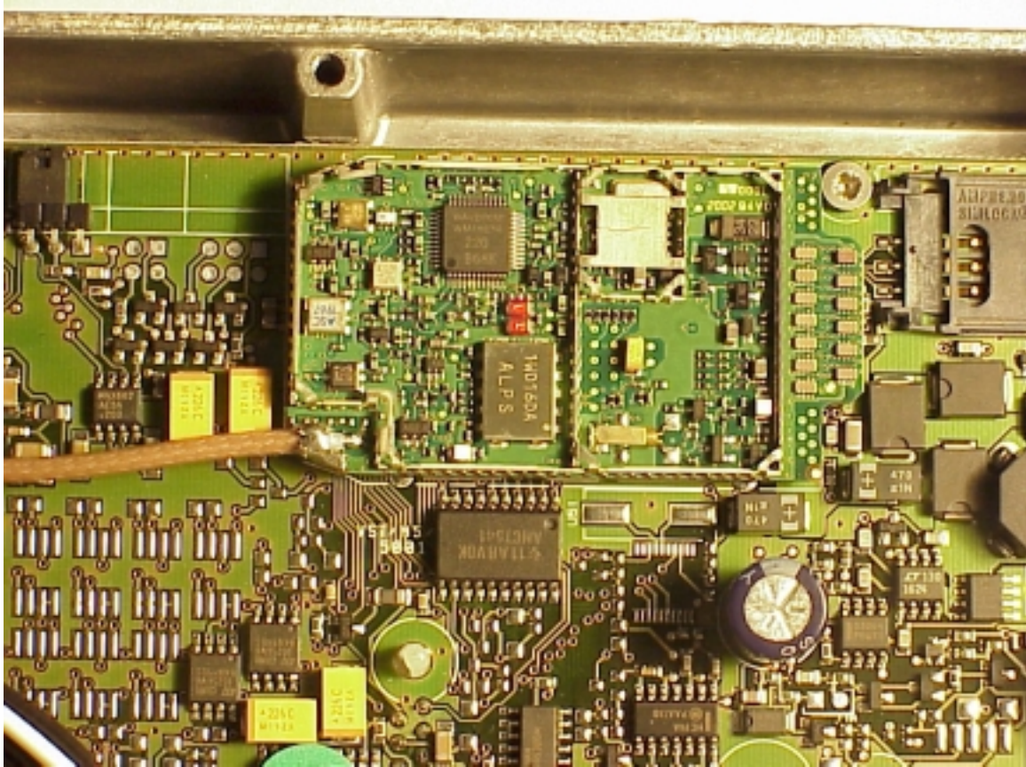
PCB – Top view unshielded (close up)
