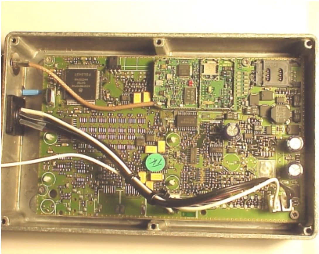
PCB – Top view unshielded
