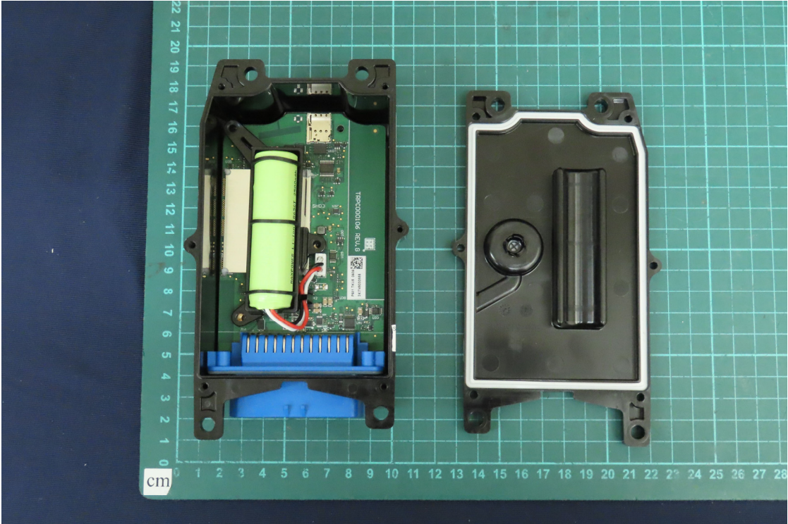
(1) EUT Photo
