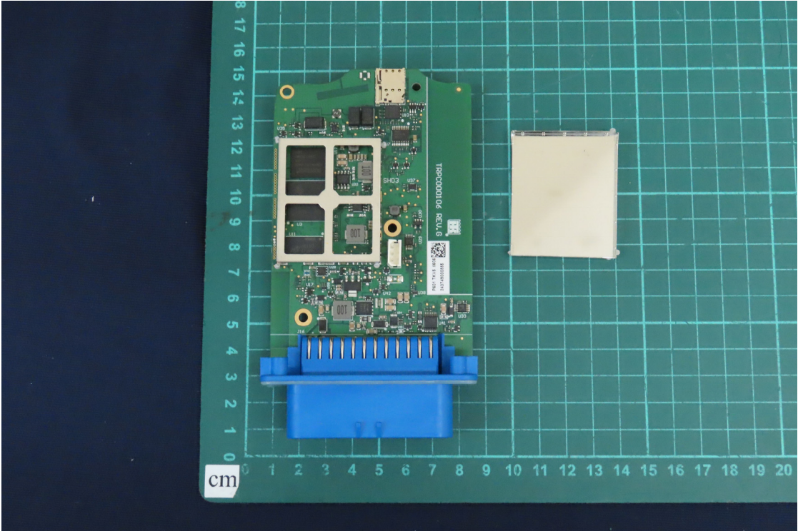
(7) EUT Photo
