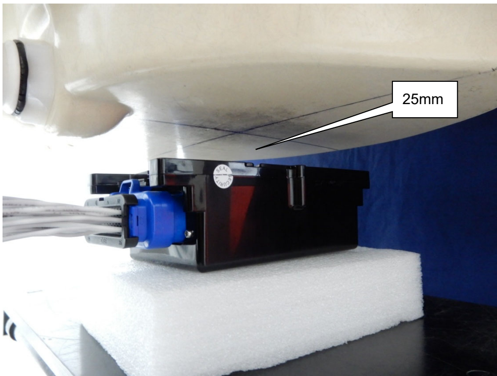
EUT Back_25mm
