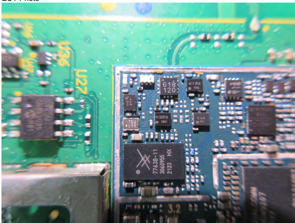
(28) EUT Photo
