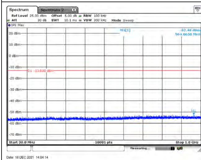
WCDMA Band 2 / RMC / 1907.6 MHz (Below 1GHz)
