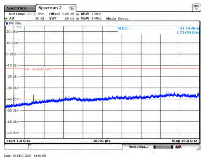
WCDMA Band 4 / RMC / 1752.6 MHz (Above 1GHz)
