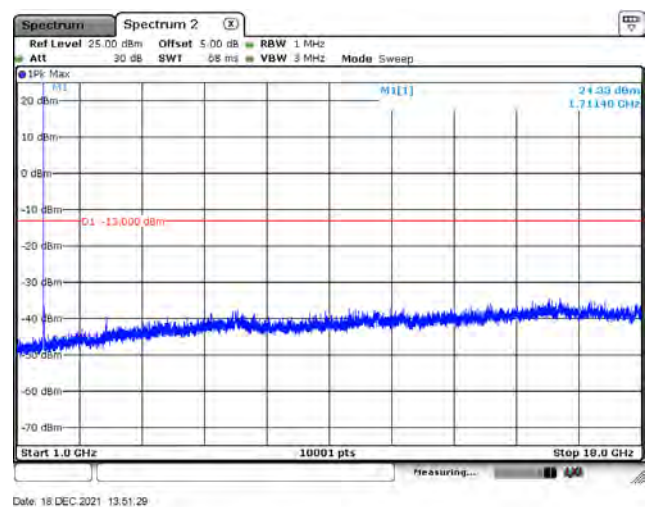
WCDMA Band 4 / RMC / 1732.6 MHz (Above 1GHz)
