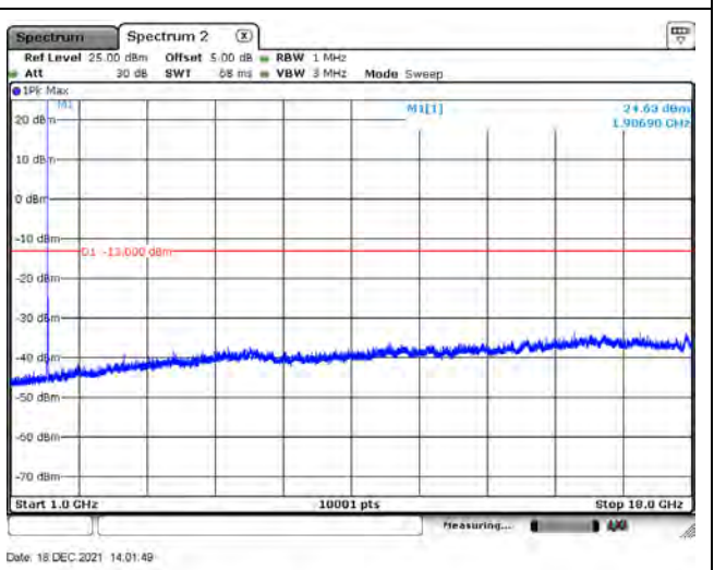
WCDMA Band 2 / RMC / 1907.6 MHz (Above 1GHz)
