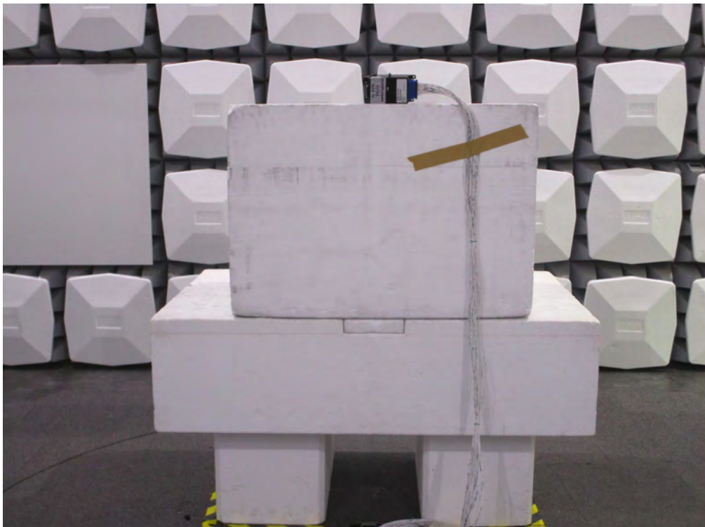
Description: Back View of Radiated Spurious Emission Test Setup (Above 1 GHz)
