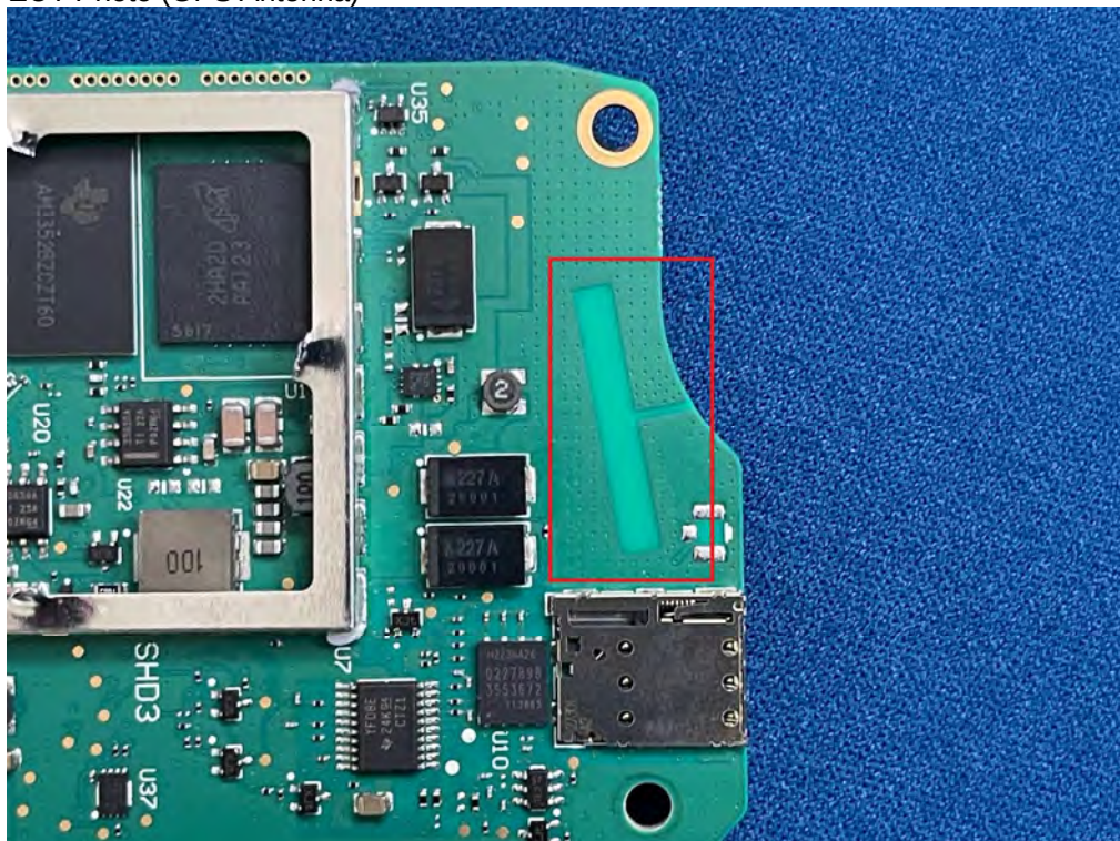
(8) EUT Photo (GPS Antenna)
