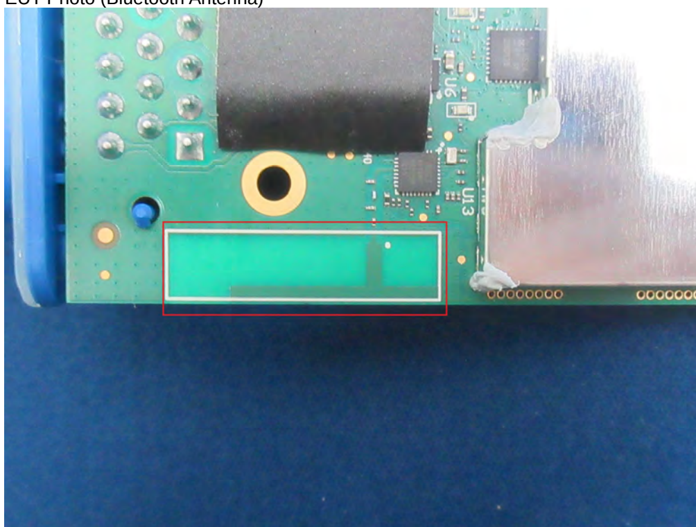
(6) EUT Photo (Bluetooth Antenna)
